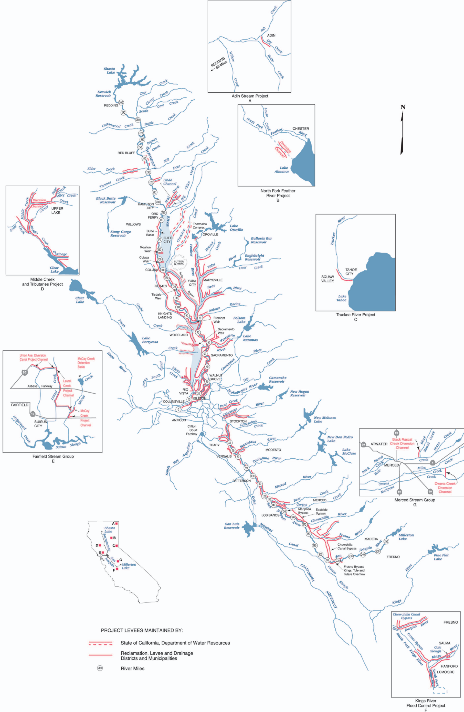
The Sacramento River and the San Joaquin River Flood Control System Project Levees and Channels
