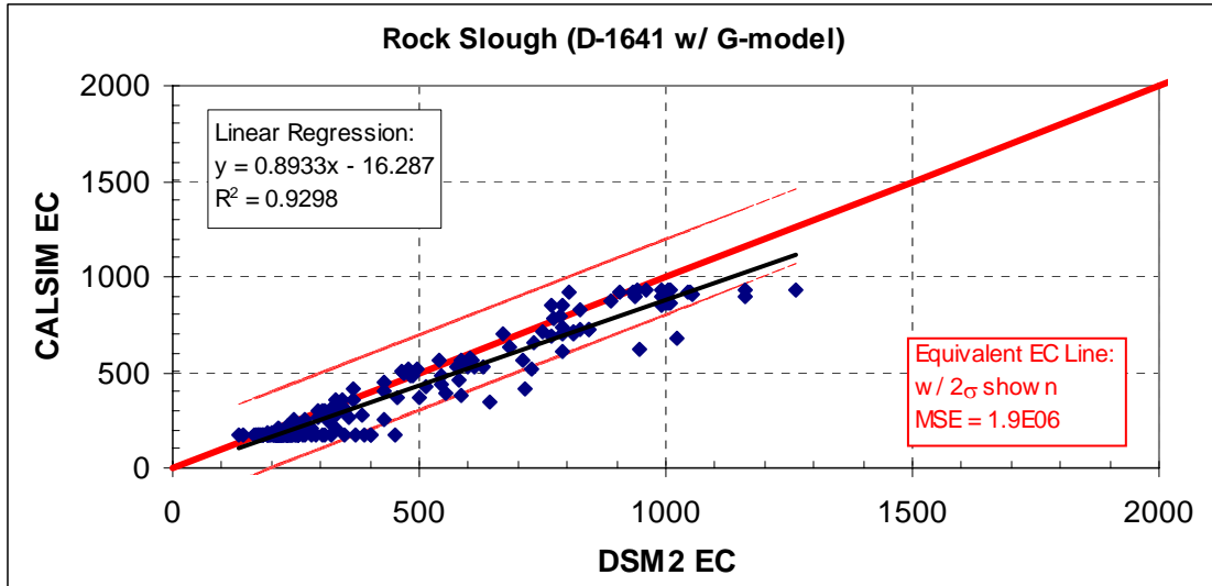
Figure 4.37: Scatter Plot of CALSIM with G-model EC versus DSM2 EC for D-1641 at Rock Slough.
