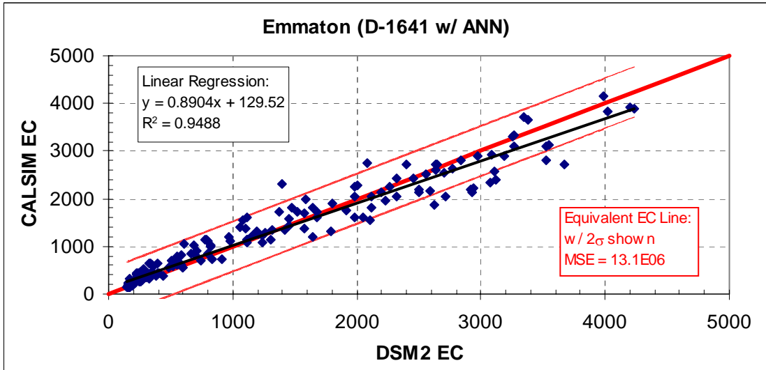
Figure 4.12: Scatter Plot of CALSIM with ANN EC versus DSM2 EC for D-1641 at Emmaton.
