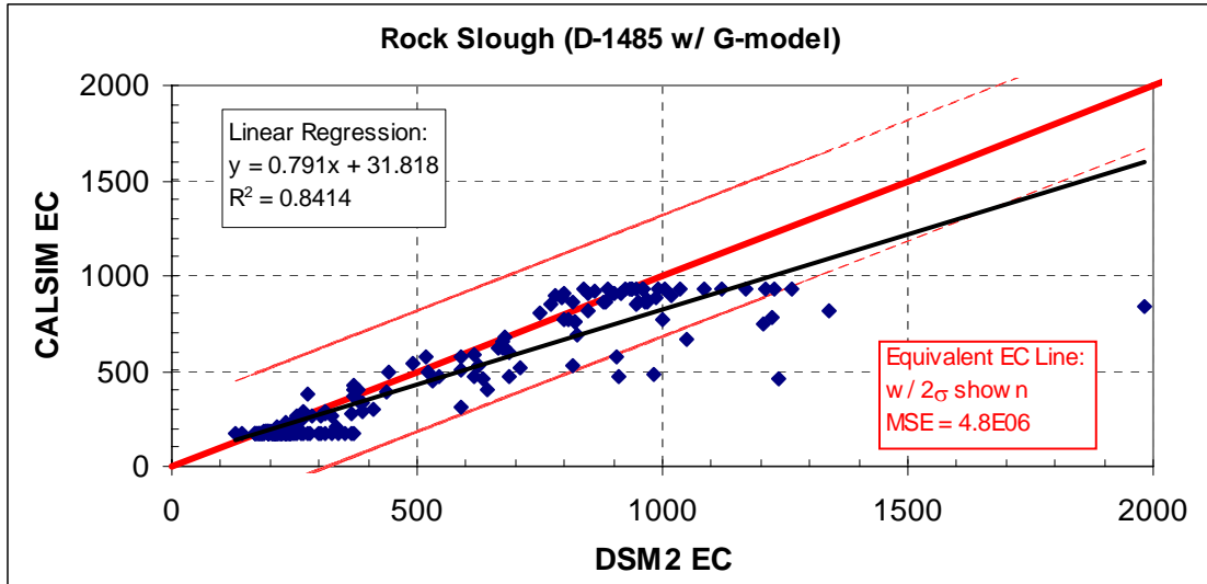
Figure 4.35: Scatter Plot of CALSIM with G-model EC versus DSM2 EC for D-1485 at Rock Slough.
