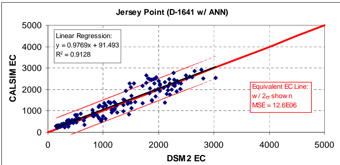
Figure 4.24: Scatter Plot of CALSIM with ANN EC versus DSM2 EC for D-1641 at Jersey Point.
