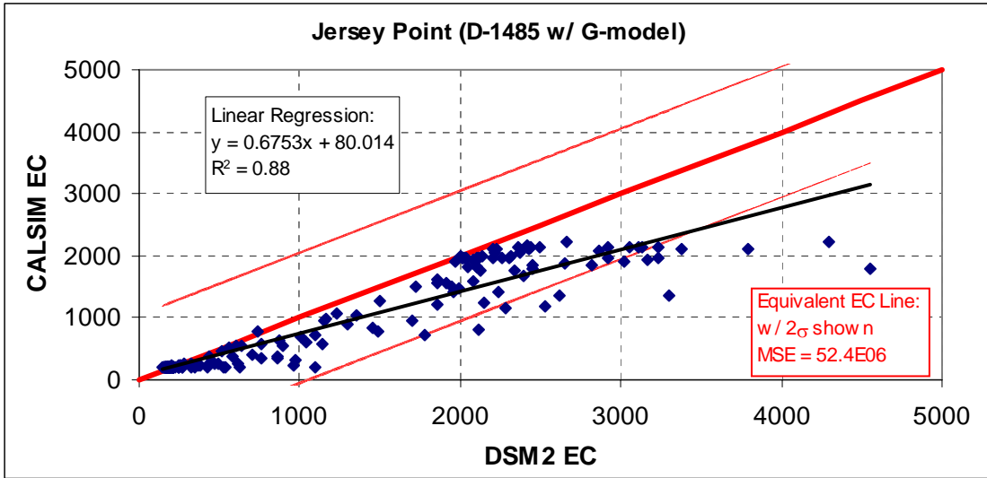
Figure 4.23: Scatter Plot of CALSIM with G-model EC versus DSM2 EC for D-1485 at Jersey Point.
