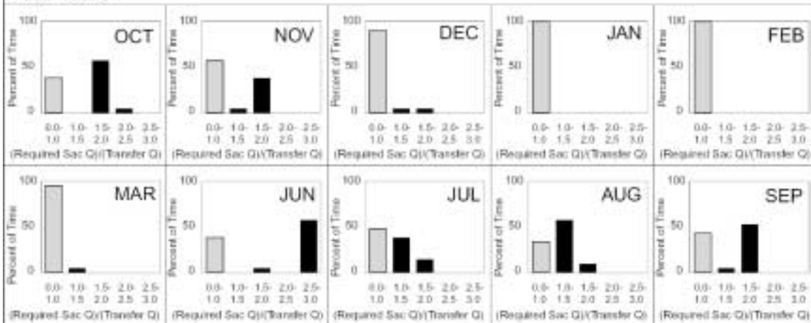
Figure 11. Distribution of Sacramento River Flow Required to Transfer 60 TAF by Month and Water Year Type (values in percent of time)
