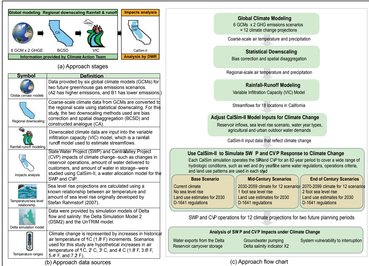
Figure 3-2 Approach used in 2009 State Water Project/Central Valley Project impact reports
