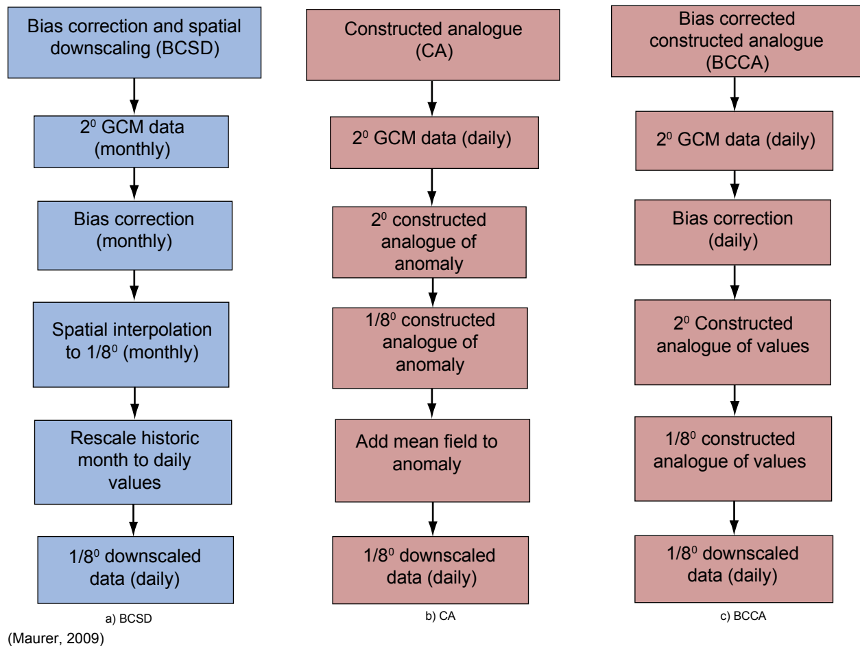
Figure 2–2 Schematics of GCM downscaling methods
